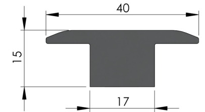
INTER CLAMP 35/40 KIT
