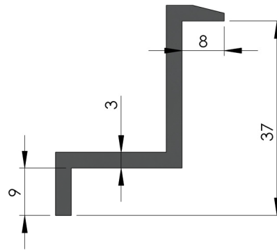
END CLAMP 35/40 KIT
