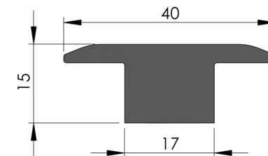
INTER CLAMP 35/40 KIT
