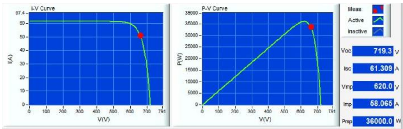
Figure 2 – DC characteristics for testing
