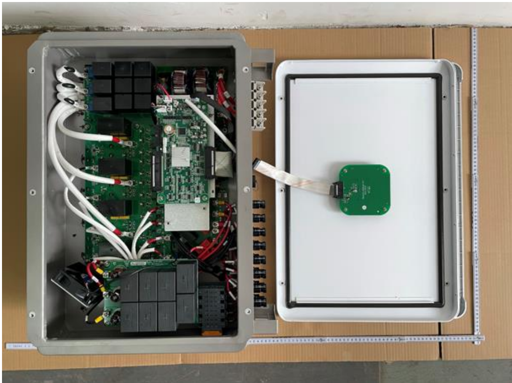
Internal view of R6-50K-T4-32, R6-40K-T4-32, R6-36K-T4-32
